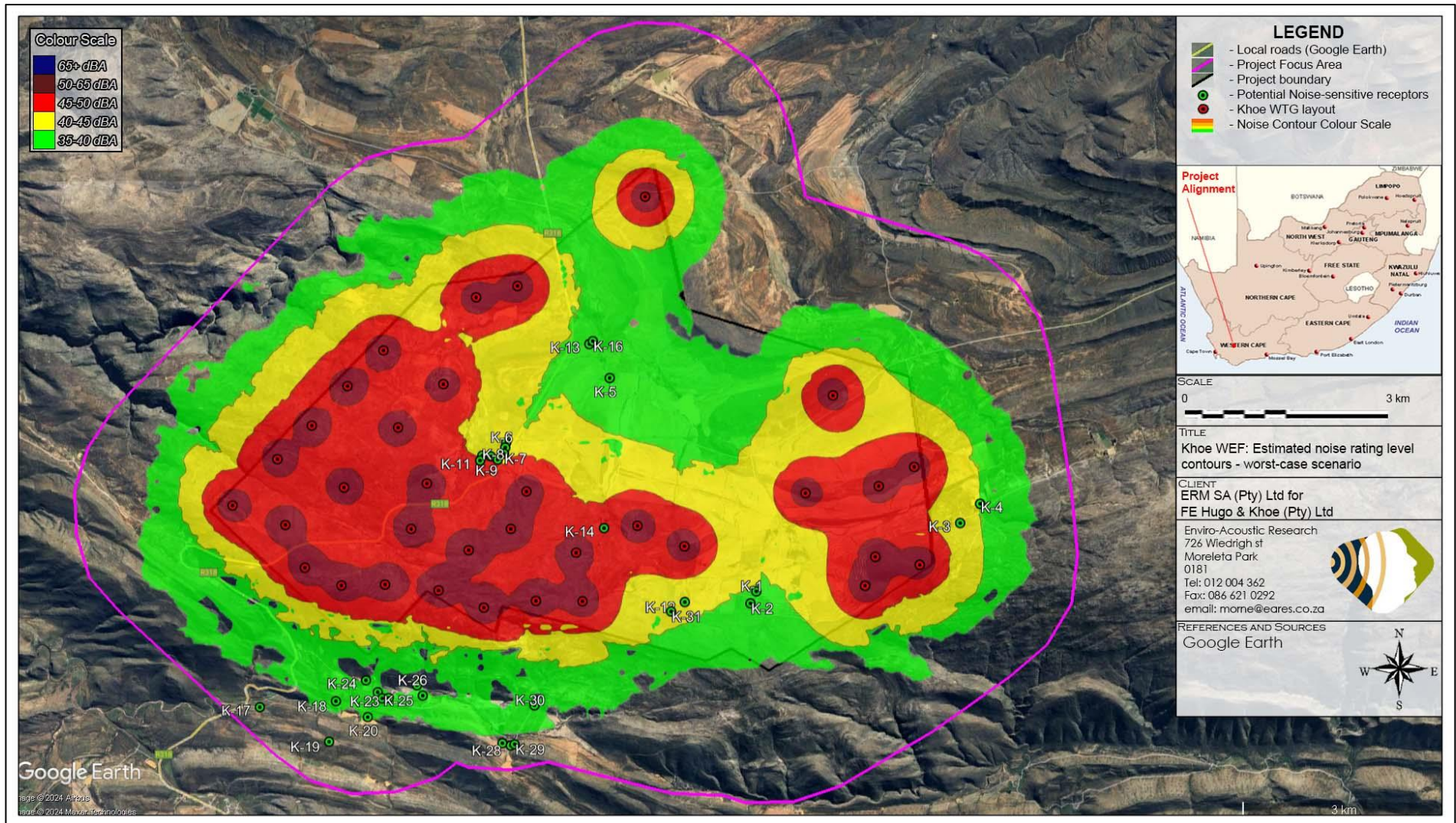
Figure 9-5: Projected future noise rating level contours – Operation of the Khoeh WEF (PWL of 108.4 dBA re 1 pW)
