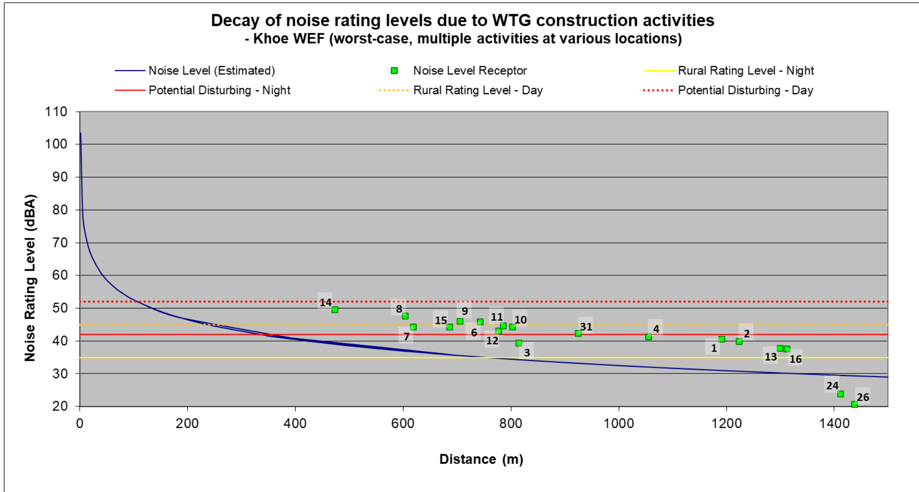
Figure 9-3: Projected conceptual construction noise levels – Khoe WEF
