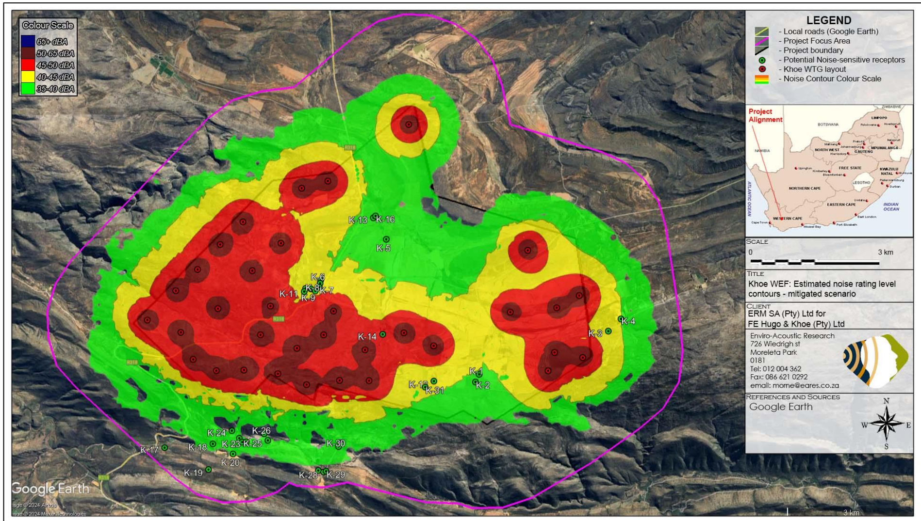
Figure 9-6: Projected future noise rating level contours – Operation of the Khoeh WEF (mitigated scenario)
