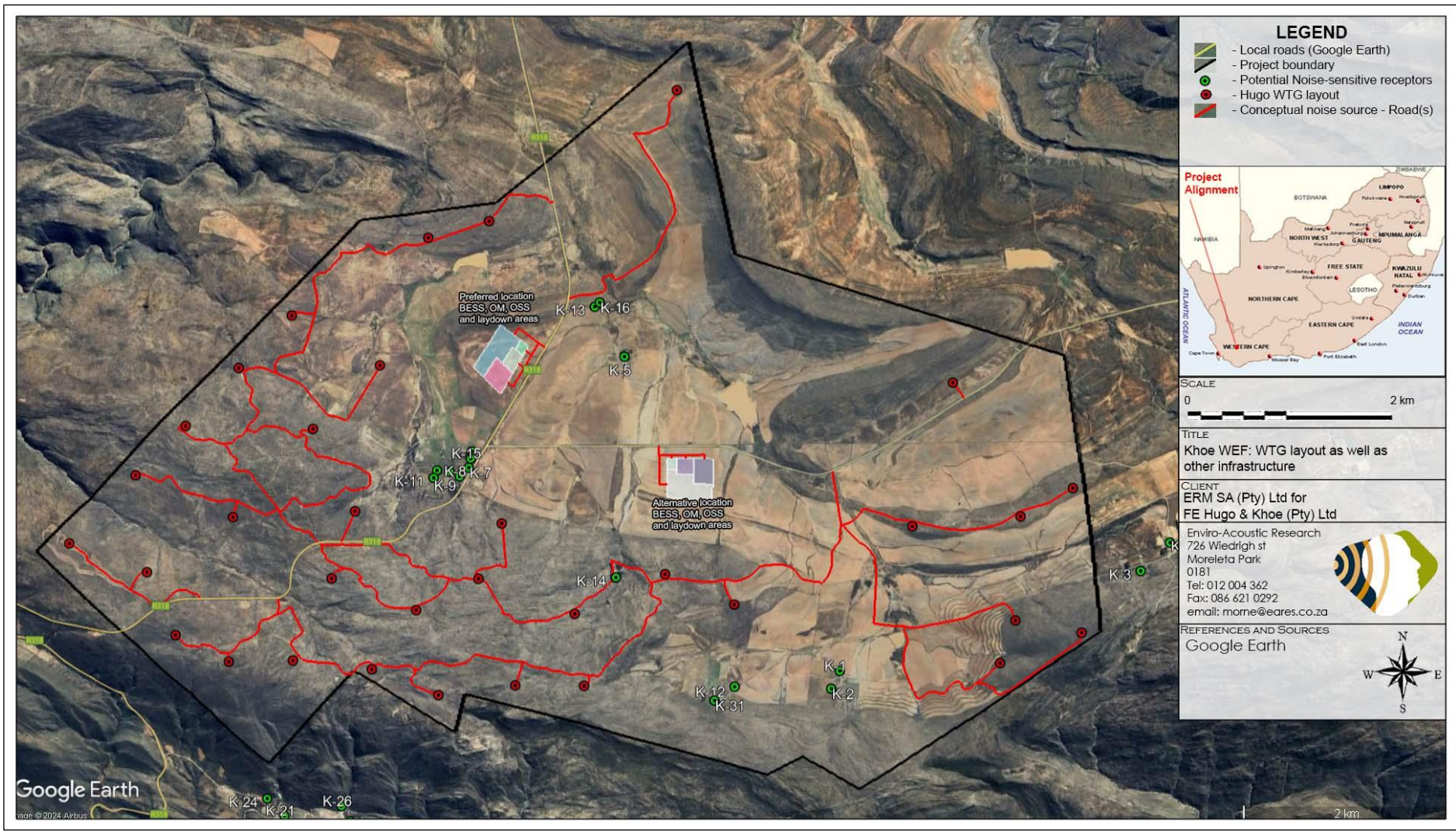
Figure 2-2: Project infrastructure of the proposed Khoe WEF
