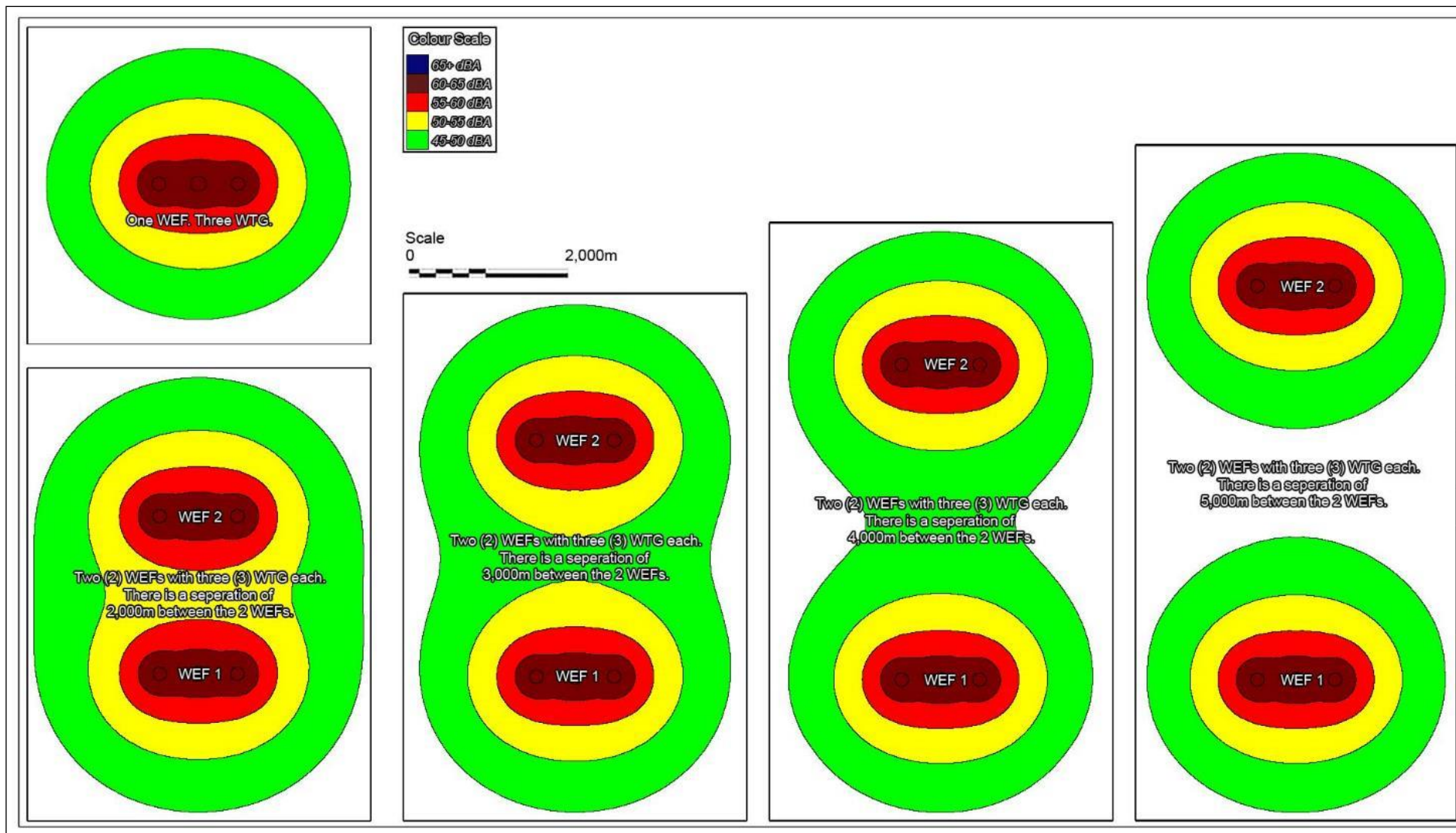
Figure 9-7: Effect of distance between wind turbines – potential cumulative noise
