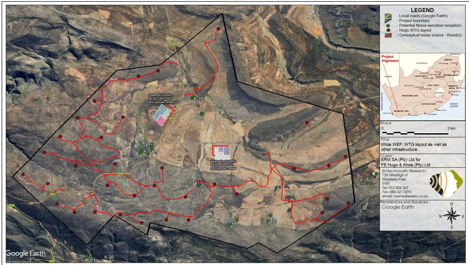
Figure 9-1: Project layout, proposed roads and other infrastructure locations for Khoe WEF
