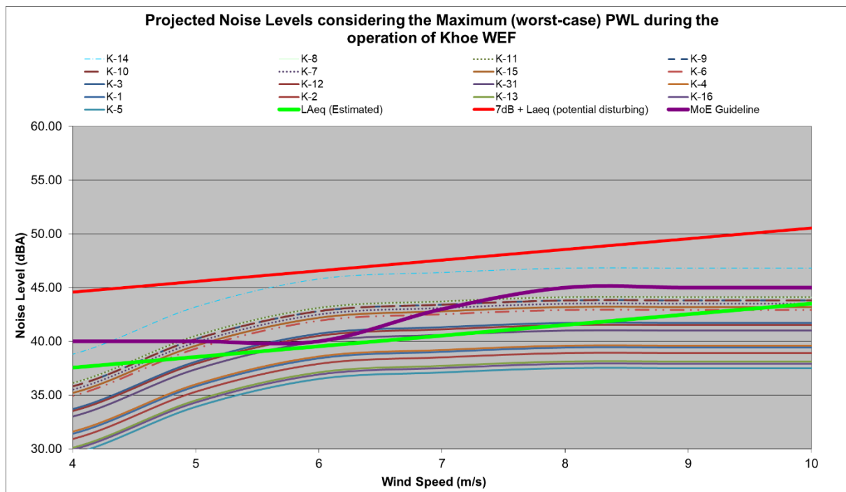
Figure 9-4: Projected noise levels at different wind speeds (worst-case PWL, with STE on blades of WTG close to Sandvlei Guest Farm)
