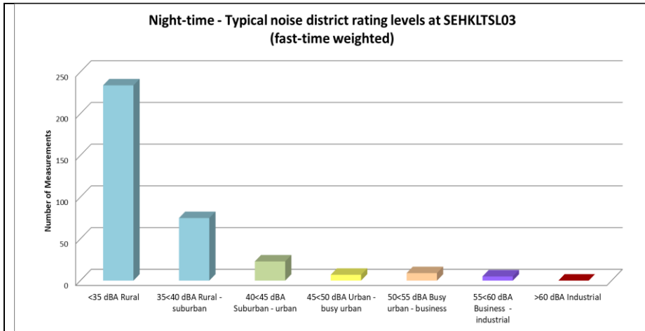
Figure 4-16: Residual noise Levels at SEHKLTSLO3
