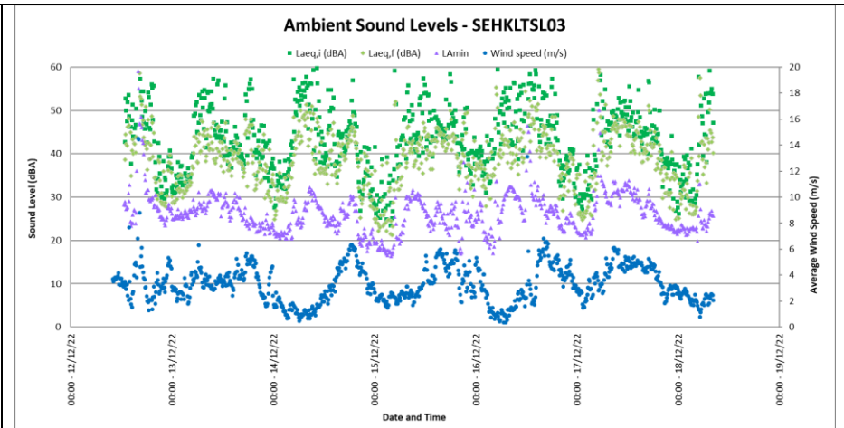
Figure 4-17: Maximum, minimum and Statistical sound levels at SEHKLTSLO3
