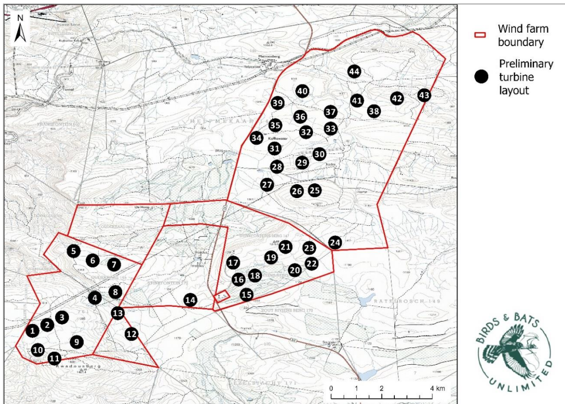
Figure 3: The 8184-ha study site (= red polygon) of the proposed HUGO Wind energy facility, 20-km south of De Doorns in the Western Cape. This map depicts the preliminary May 2023 turbine layout (black circles), and these have now changed in line with the recommendations in this report (see Figures 14(a), 14(b) and the new layout revised in March and July 2024.
