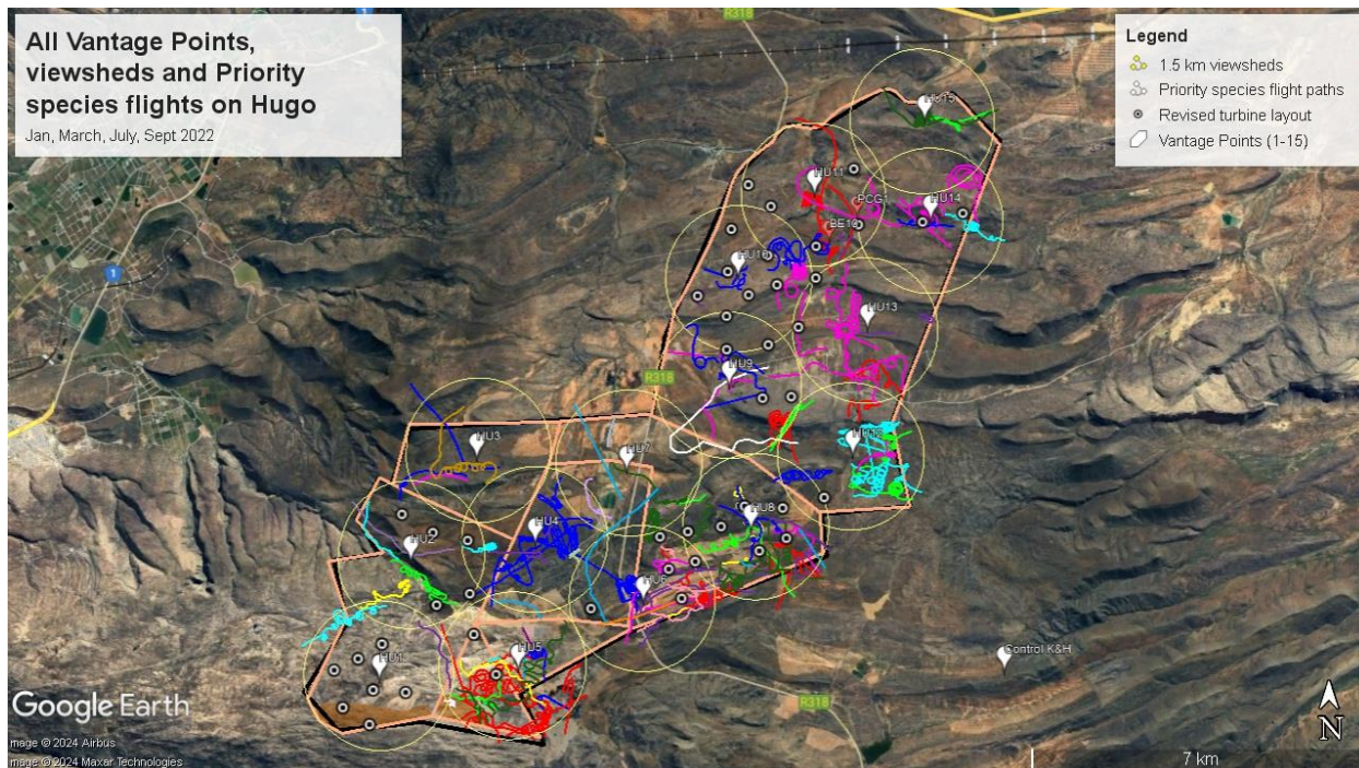
Figure 4: The proposed HUGO Wind energy facility, indicating all Vantage Points (= white balloons), associated 1.5-km viewsheds (= yellow circles), and the revised (46) turbine positions (= small black/white circles). All priority species flights recorded over 12 months to indicate the density of movements, used as the basis for the CRM/FRM modelling to follow.
